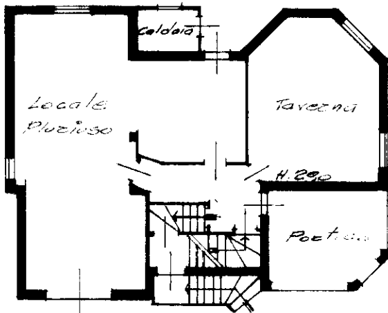
PIANO TERRENO
